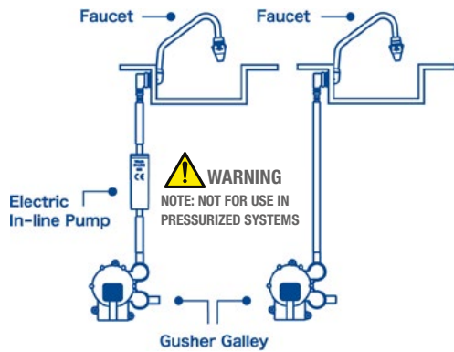
TYPICAL INSTALLATION
